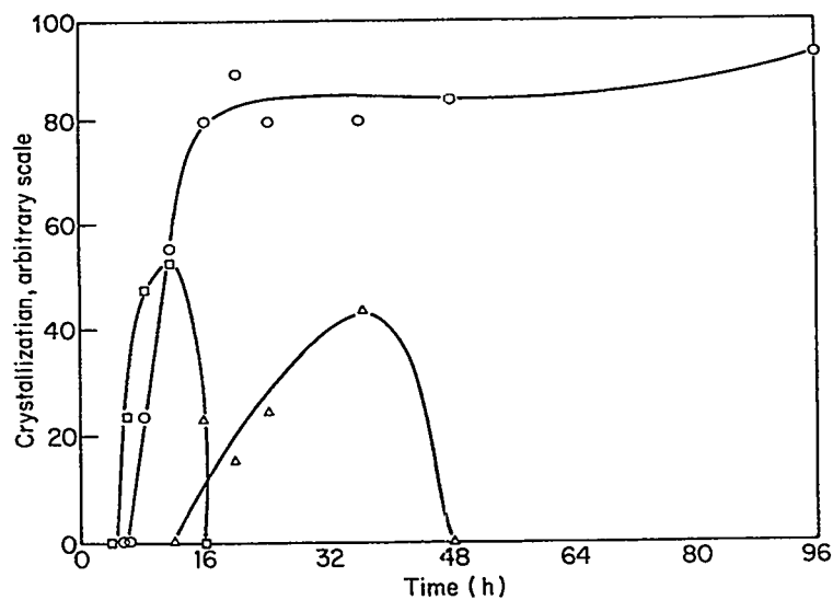
Crystallization curves showing appearance and disappearance of mordenite ( \square ) and an analcime type phase ( \Delta ) during growth of zeolite ZSM-5 ( \circ ) from the parent composition 6(\text{TPA})_2 \cdot 4\text{Na}_2\text{O} \cdot \text{Al}_2\text{O}_3 \cdot 28\text{SiO}_2 \cdot 750\text{H}_2\text{O} . After Erdem and Sand (1979).
