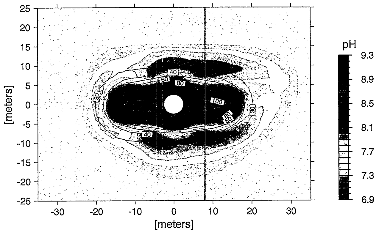
Figure 3.3-7. pH in fractures after 6 months of heating. Temperature contours are overlain.
