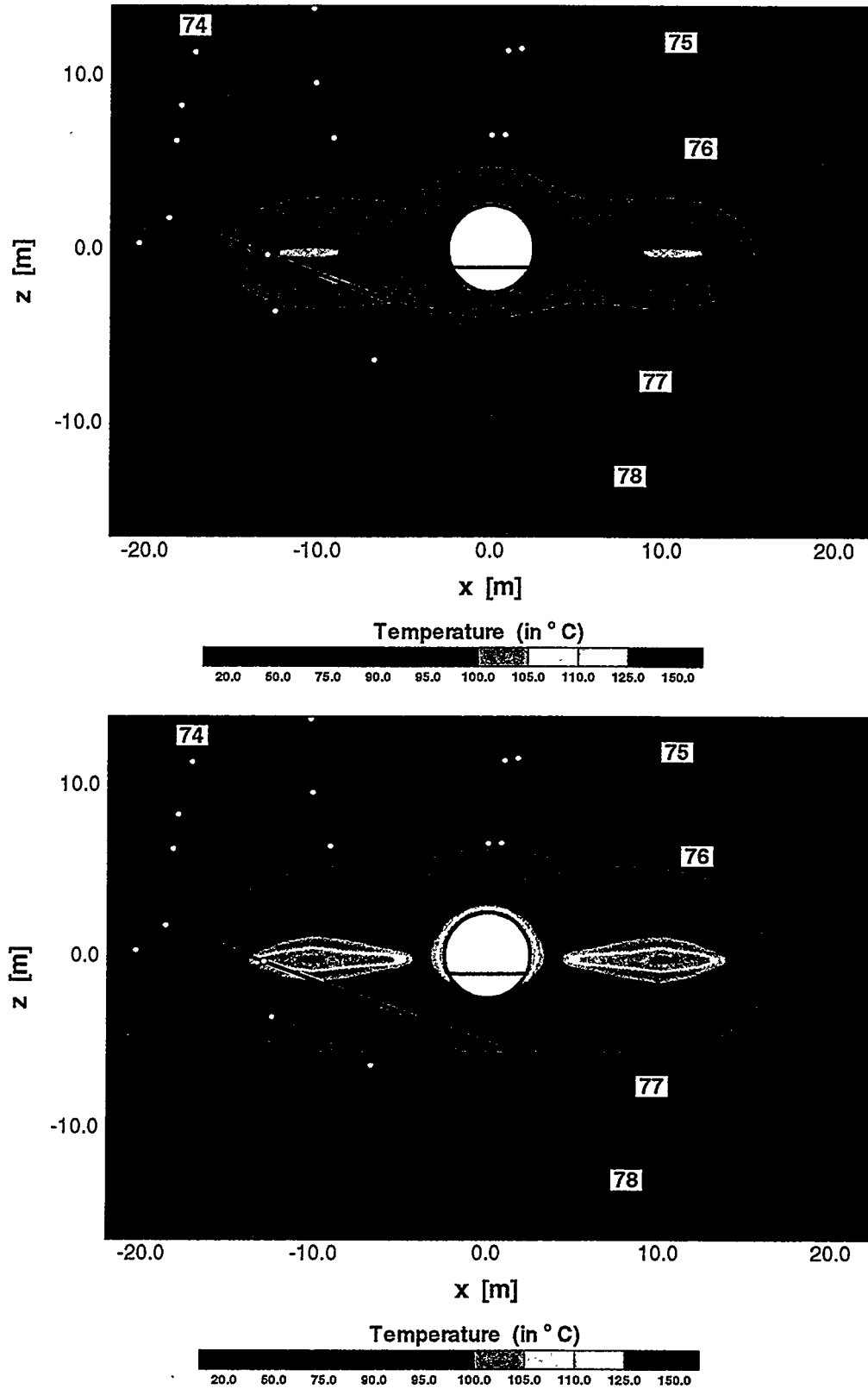
Figure 2.7. Simulated temperature response at 3 months (top) and 6 months (bottom) of heating in xz-cross section at y = 30 m.
