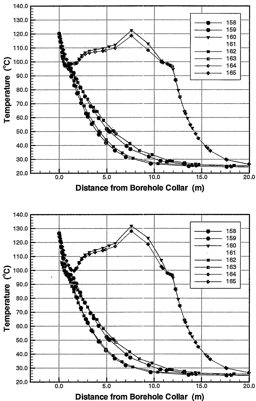
Figure 2.28. Simulated temperature profiles along boreholes 158 to 165 at 6 months of heating, using a 3.6 mm/yr percolation flux (top) and a 0.36 mm/yr percolation flux (bottom).
