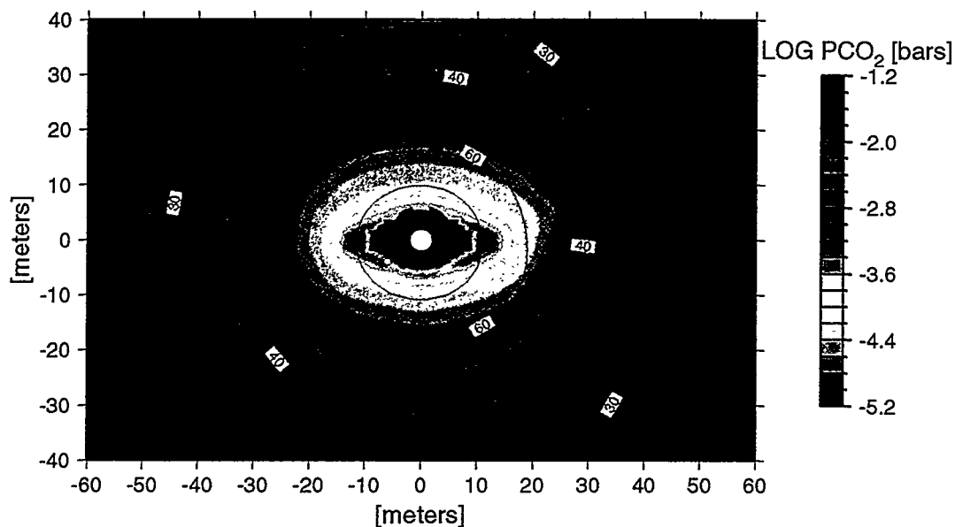
Figure 3.3-6. Partial pressure of CO 2 in fractures at the end of the 8 year heating and cooling cycles. Temperature contours are overlain.
