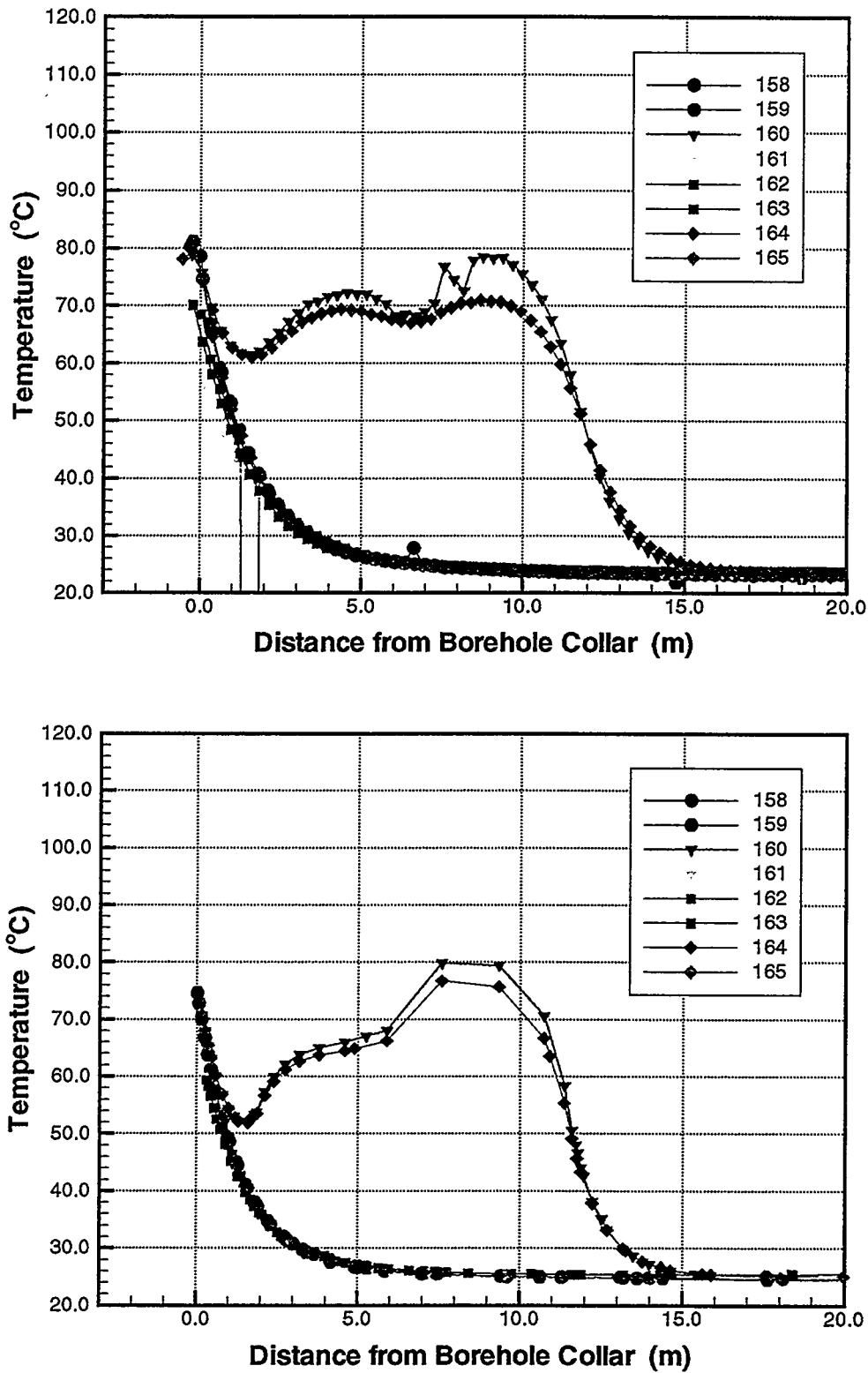
Figure 2.11. Measured (top) and simulated (bottom) temperature profiles along boreholes 158 to 165 at 1 month of heating
