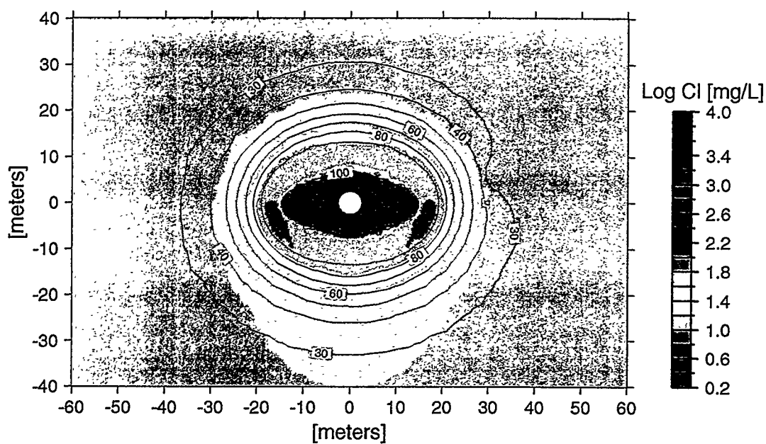
Figure 3.3-2. Chloride concentration in fractures at the end of the 4 year heating cycle. Temperature contours are overlain.
