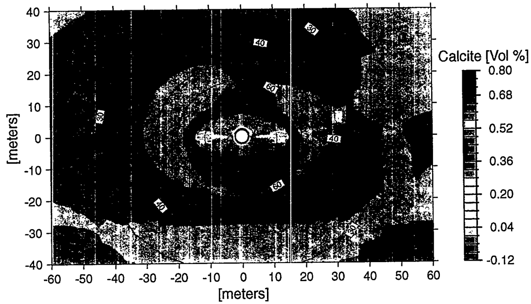
Figure 3.3-10. Calcite volume fraction dissolved/precipitated in fractures at the end of the 8 year heating and cooling cycles. Temperature contours are overlain.
