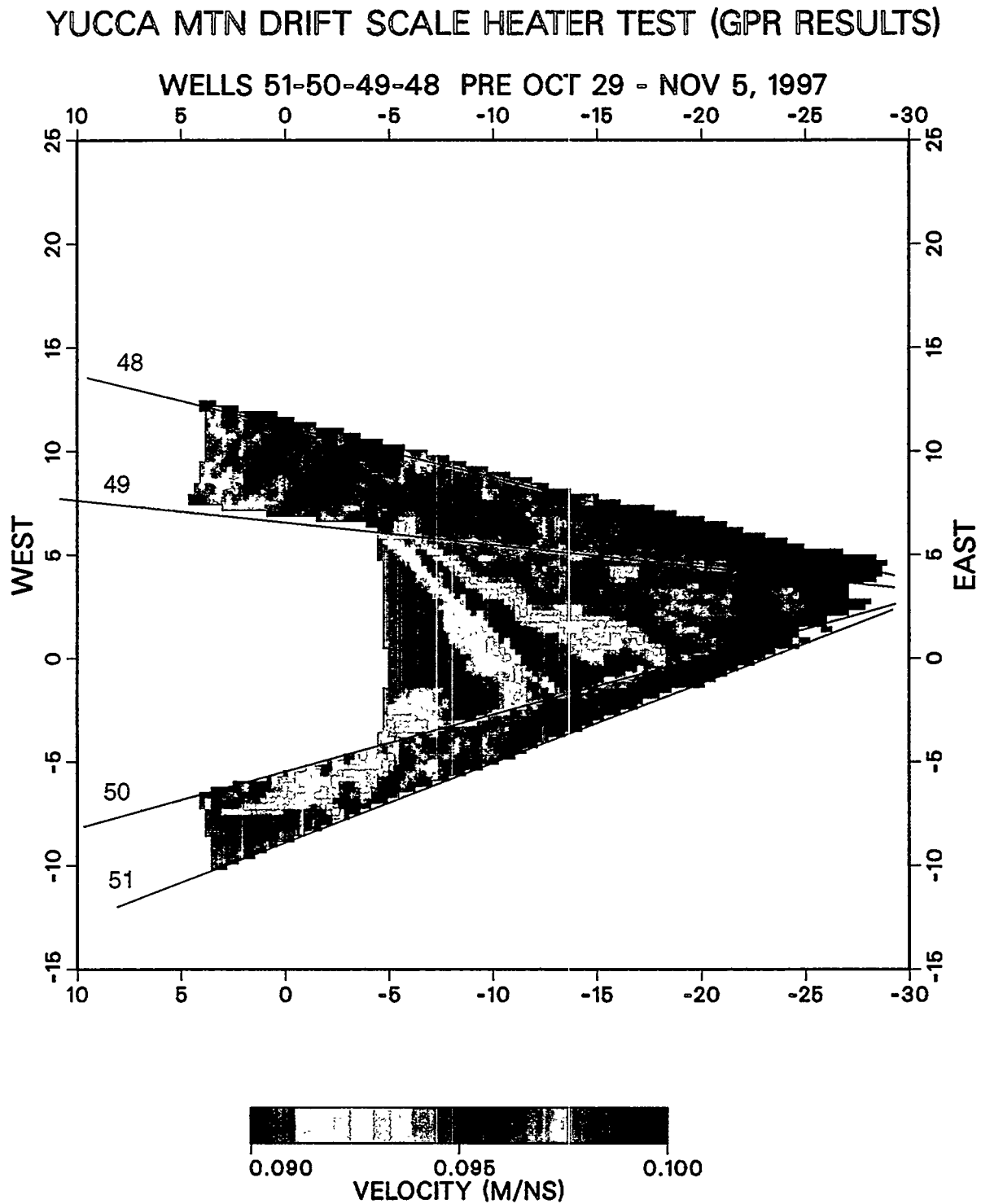
Figure 4.1. Velocity tomogram in the 51-47 plane for the Pre-heat baseline data.
