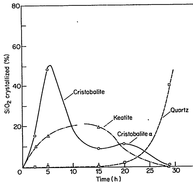
Transformation of amorphous \text{SiO}_2 to quartz, cristobalite, and keatite as a function of time. Temperature 300^\circ\text{C} , in presence of 3% KOH aq., after Siffert and Wey (1967).
