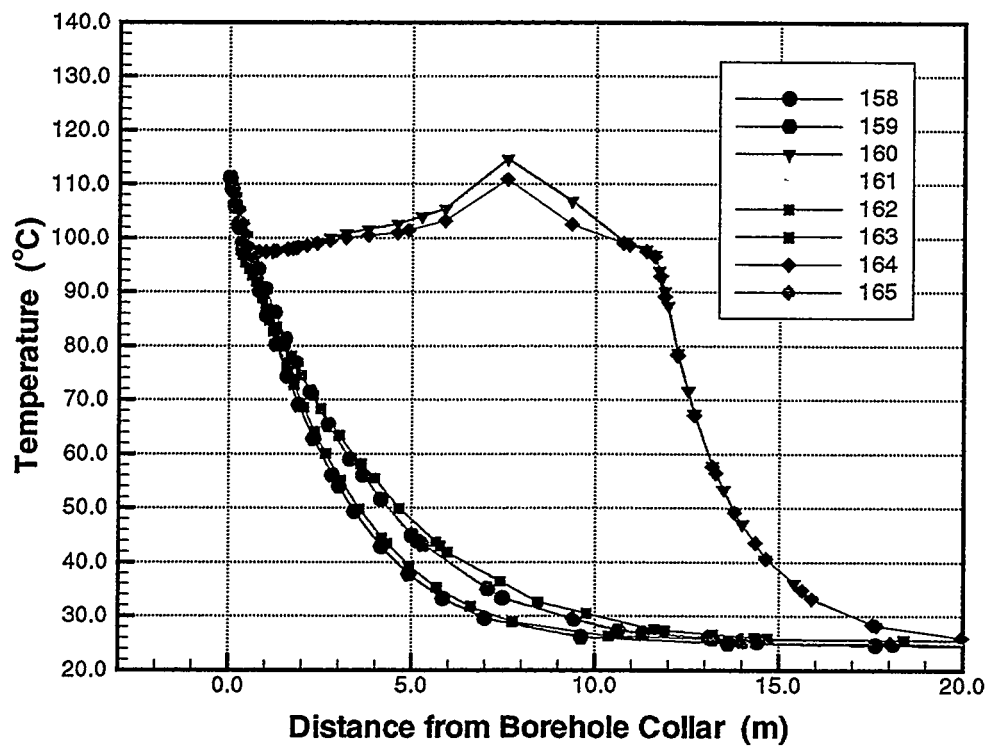
Figure 2.15. Measured (top) and simulated (bottom) temperature profiles along boreholes 158 to 165 at 5 months of heating.
