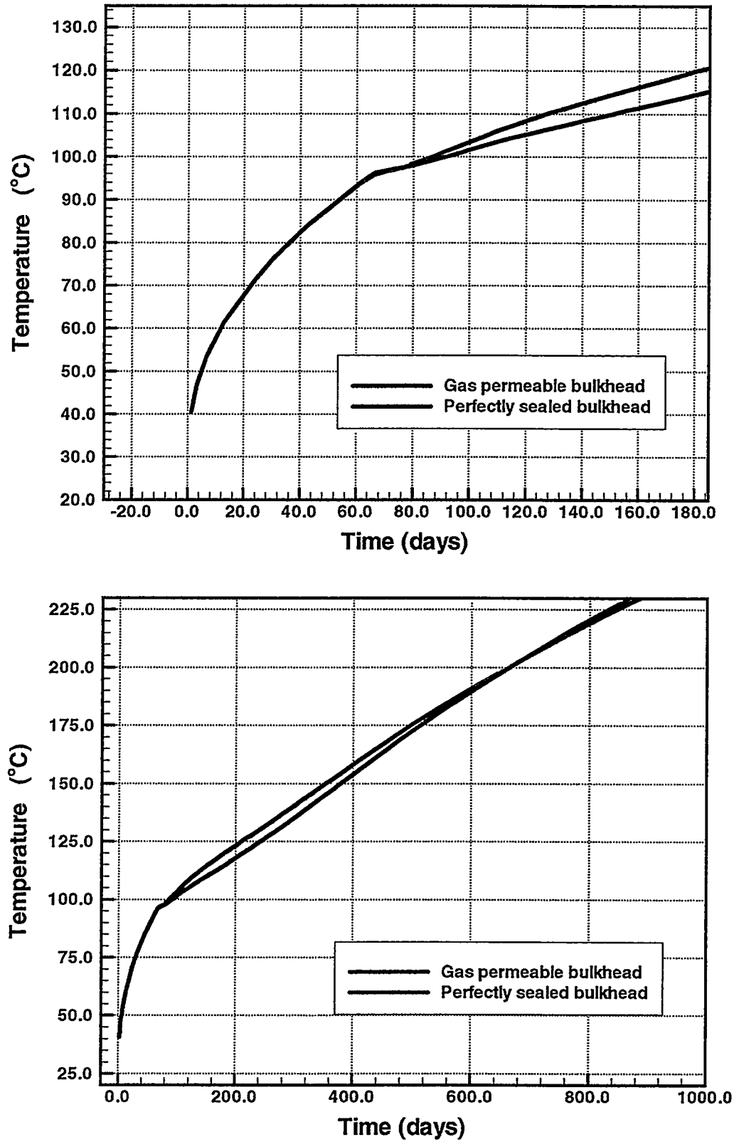
Figure 2.25. Simulated temperature evolution at the Heated Drift wall for alternative bulkhead boundary conditions up to 185 days (top) and up to 1000 days (bottom).
