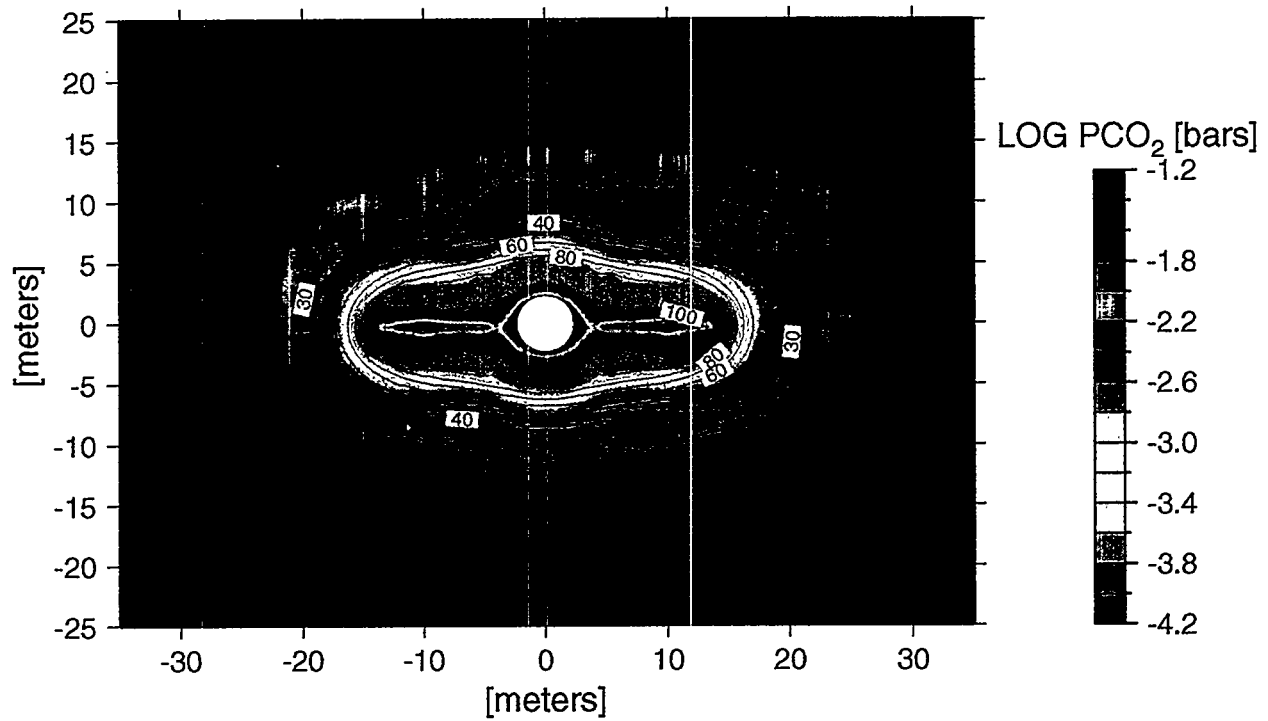
Figure 3.3-4. Partial pressure of \text{CO}_2 in fractures after 6 months of heating. Temperature contours are overlain.
