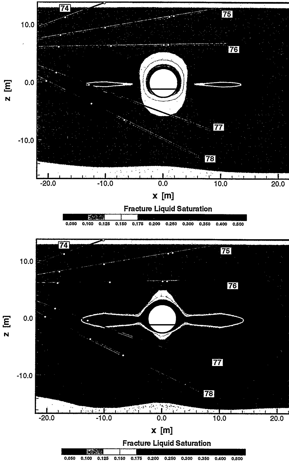
Figure 2.9 Simulated fracture saturation at 3 months (top) and 6 months (bottom) of heating in xz-cross section at y = 30 m.
