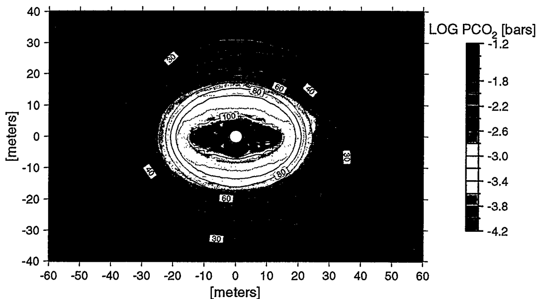
Figure 3.3-5. Partial pressure of CO 2 in fractures at the end of the 4 year heating cycle. Temperature contours are overlain. Irregularities in the temperature profile to the right of the drift are due to the constant temperature observation drift.
