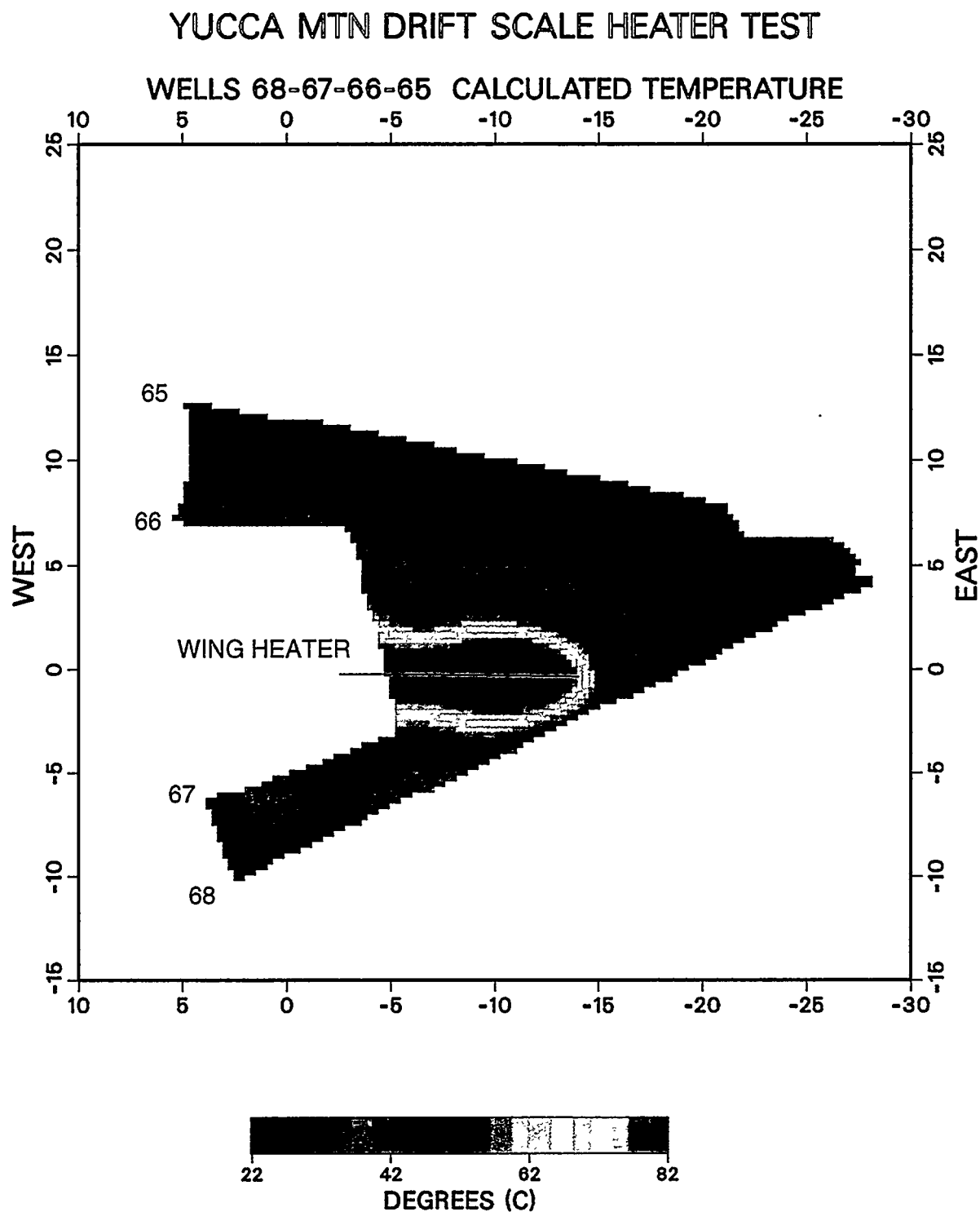
Figure 4.9. Temperature profile for the 64-68 plane as interpolated from the temperature model of Birkholzer and Tsang (1998).
