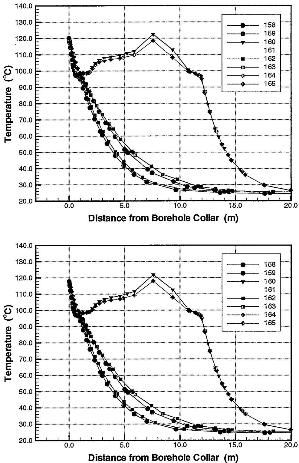
Figure 2.26. Simulated temperature profiles along boreholes 158 to 165 at 6 months of heating, with initial drying due to ventilation (top) and without initial drying (bottom).
