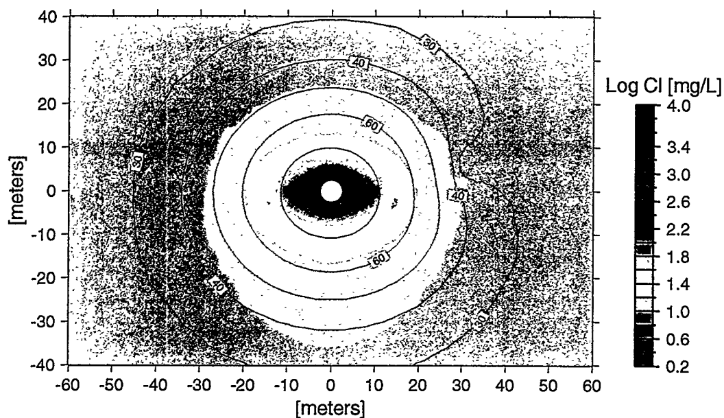
Figure 3.3-3. Chloride concentration in fractures at the end of the 8 year heating and cooling cycles. Temperature contours are overlain.
